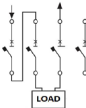
3 poles in series
